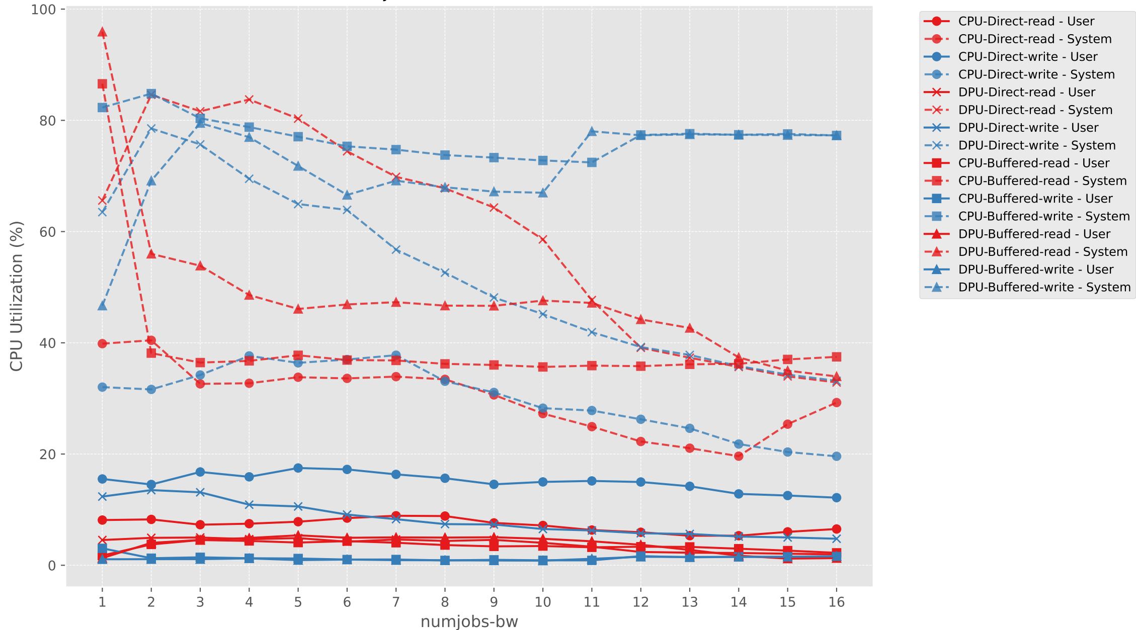
CPU Utilization vs numjobs-bw (CPU vs DPU, Direct vs Buffered)
